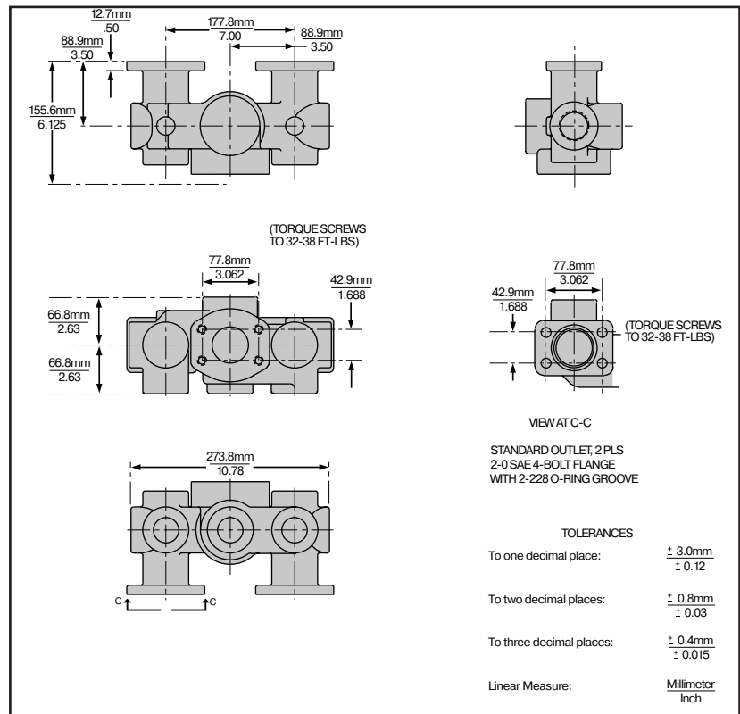
INSTALLATION DIMENSIONS
