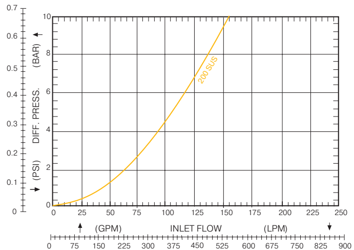
Flow/Pressure Curve
