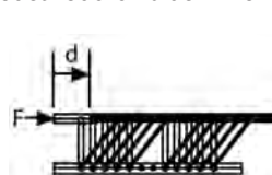
FIXED SHEAR (for Wire Rope Isolators)
