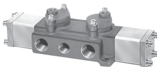
1/2" Basic, Nominal Cv = 5.2
