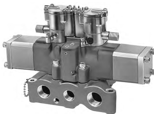
1" Basic, Nominal Cv = 11.3
