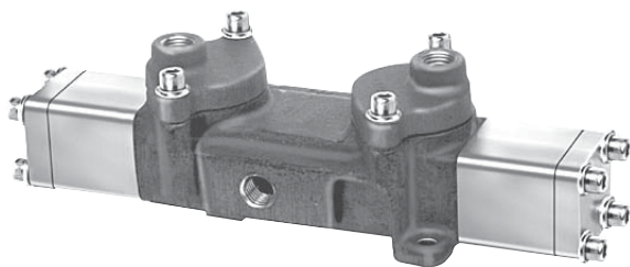
1/4" Basic, Nominal Cv = 1.7
