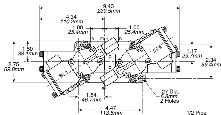
1/4" Basic
